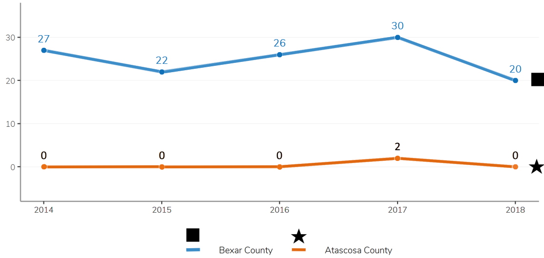
Fig. 7.9 Traffic accidents causing incapacitating injuries for cyclists
