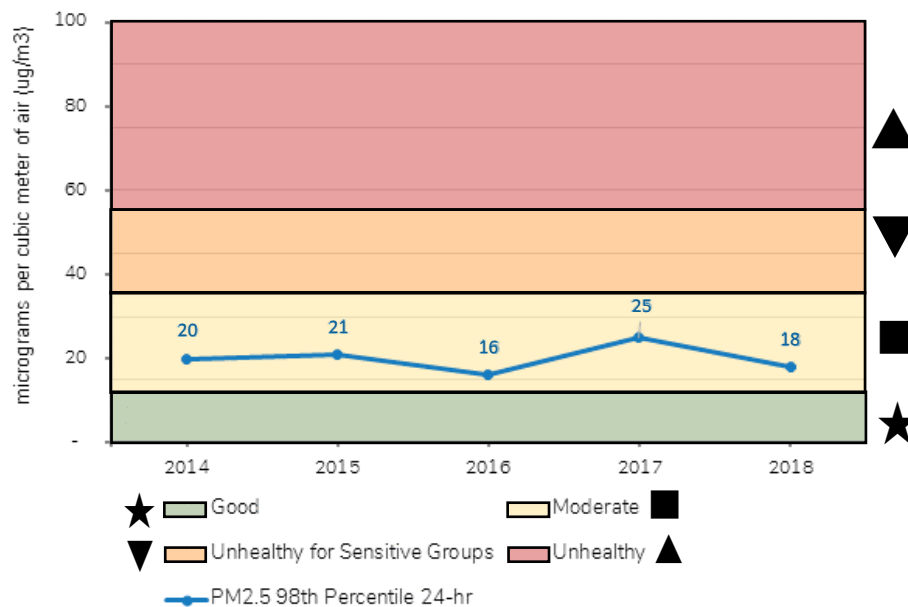
Fig. 2.1.2 98th percentile 24-hr PM 2.5 reading in San Antonio
